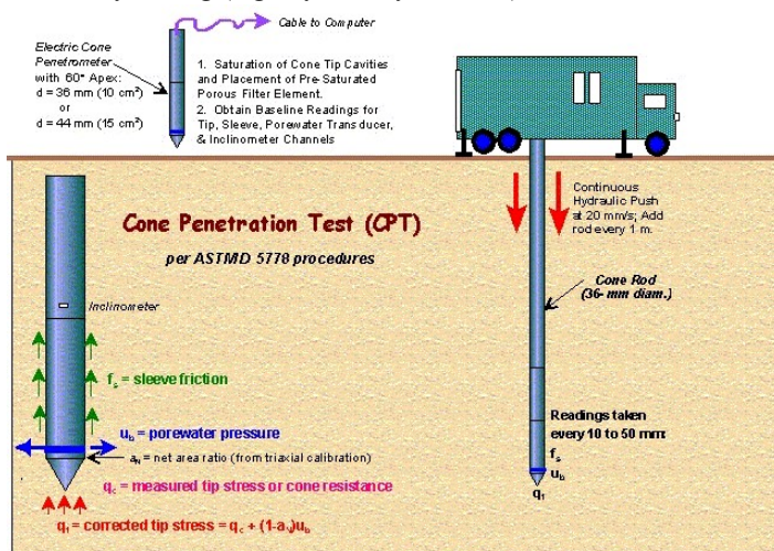
Fig. 1 General concept of CPT testing (Patrick, 2008)
